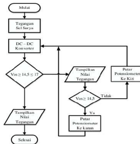
Gambar 2. Diagram alir prinsip kerja rangkaian controller fast charging
