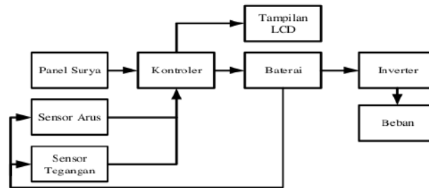
Gambar 1. Block Diagram Perancangan
