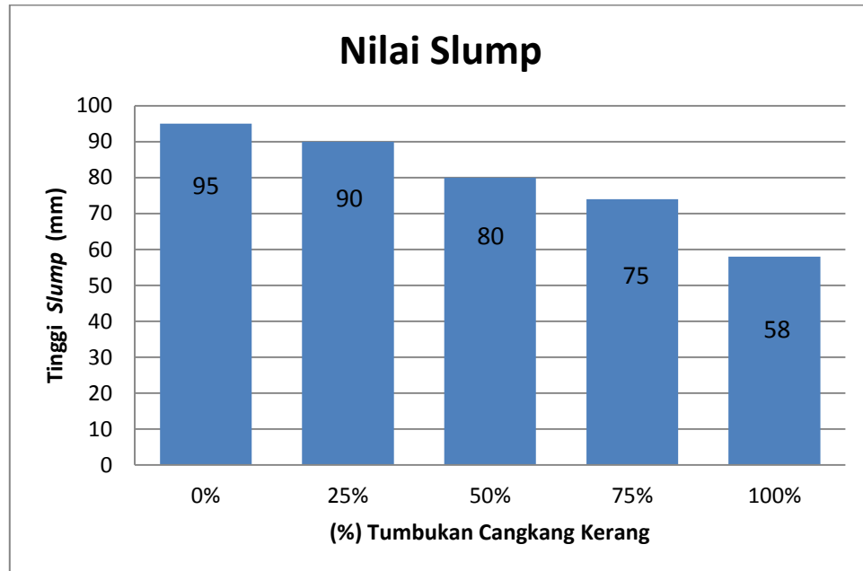
Gambar 4.12 Nilai Slump
