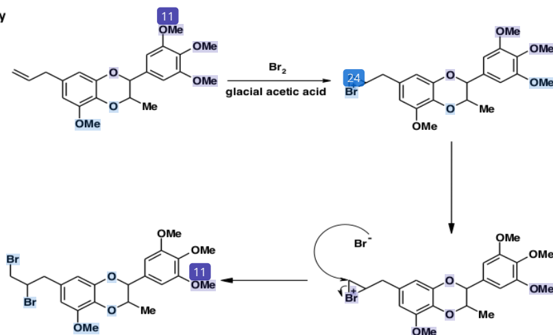
Figure 2. Synthesis of Eusiderin A dibromide
