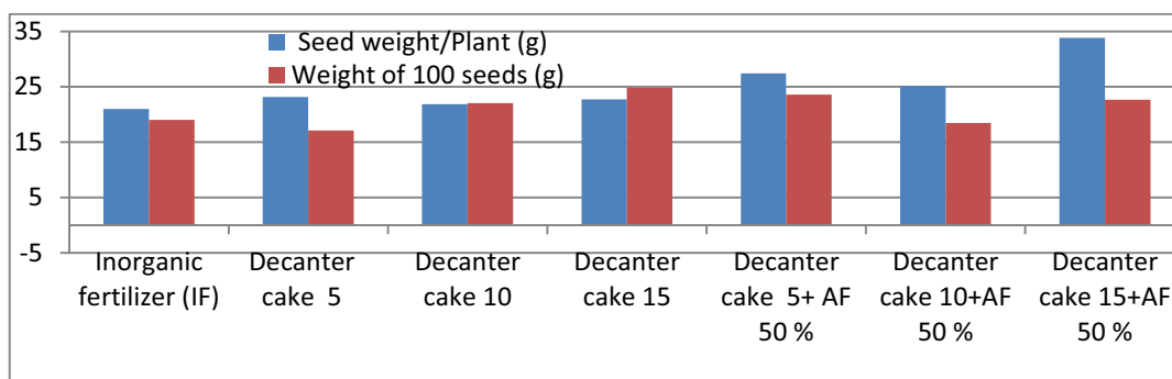
Figure 2. Effects of fertilizer differences on seed weight per plant and 100 seed weight
