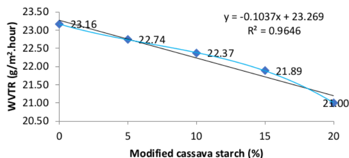
Figure 4. WVTR edible film at several levels of modified starch concentration
