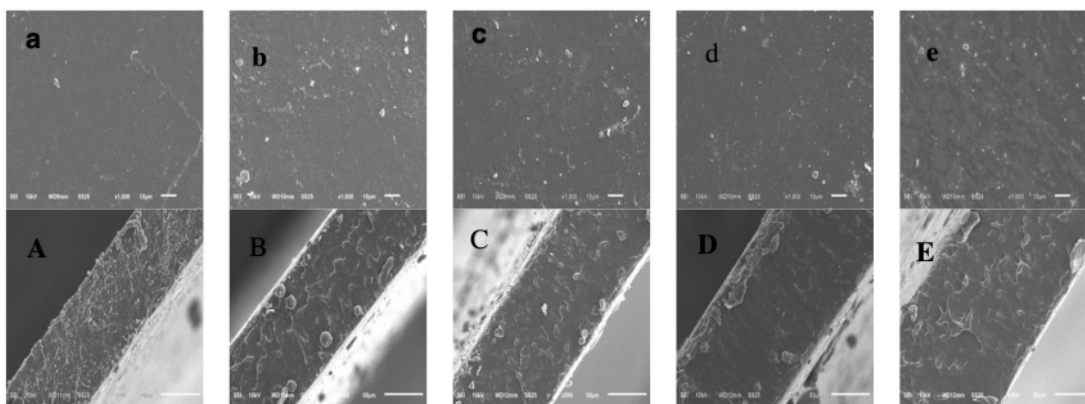
Figure 2. SEM image of surface and cross-section of edible film with various concentrations of modified starch at 500x magnification. Film surface 0% (a), 5% (b), 10% (c), 15% (d), and 20% (e), Film cross-section 0% (A), 5% (B), 10% (C), 15% (D), and 20% (E)
