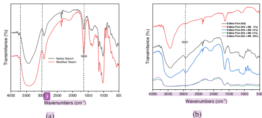
Figure 3. FTIR spectra of starch (a) and edible film (b) where NS: Native Starch, MS: Modified Starch
