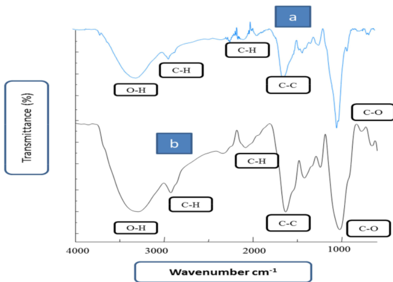
Figure 2. FTIR Spectra of CRI-WAS adsorbents (a) before, (b) after Cd(II) is loaded
