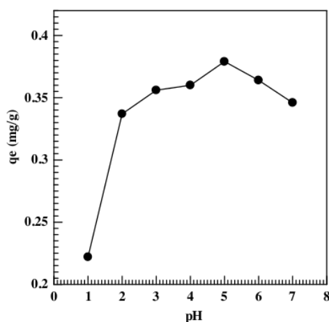
Figure 3. Effect of pH solution on adsorption capacity of Cd(II) by CRI-WAS adsorbent
