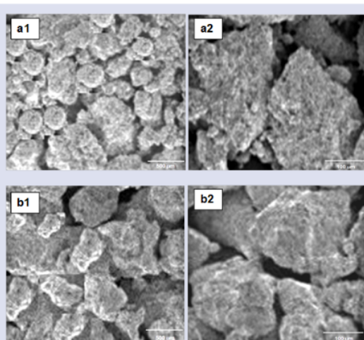
Figure 3: SEM (Scanning Electron Microscope) Eudragit E100 and Ethocel 10 cP polymer microparticles at magnifications of 100x and 650x. a). Eudragit E100 (15%, FA3) and b). Ethocel 10 cP (15%, FB3), 1) magnifications of 100x and 2) magnifications of 650x.
